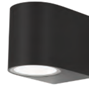
CH-03 BLACK 42-0032 H9 x 7 x 8 cm GU10 LED max 5W IP44
